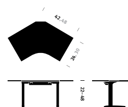
120° Corner Table with C-Foot
